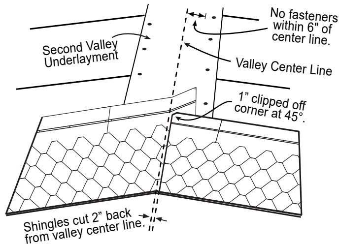
Figure 4 Closed-Cut Valley
