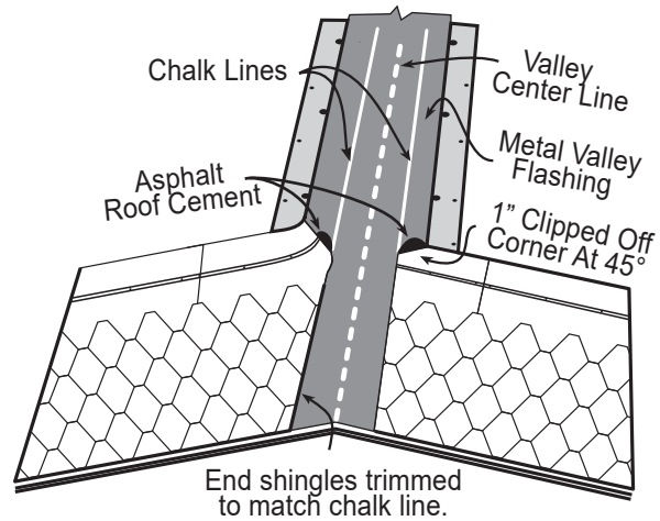
Figure 3 Shingle Application
