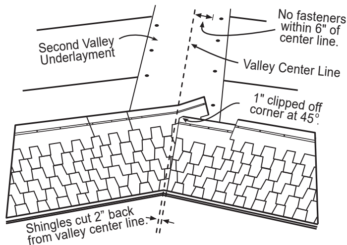
Figure 4 Closed-Cut Valley
