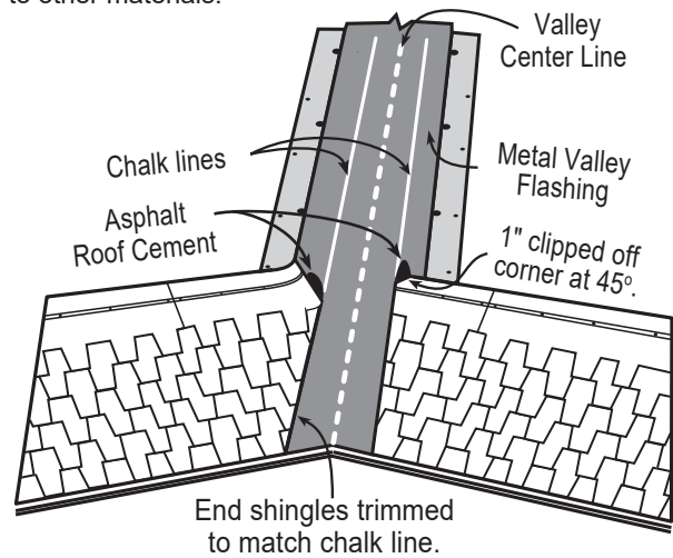
Figure 3 Shingle Application
